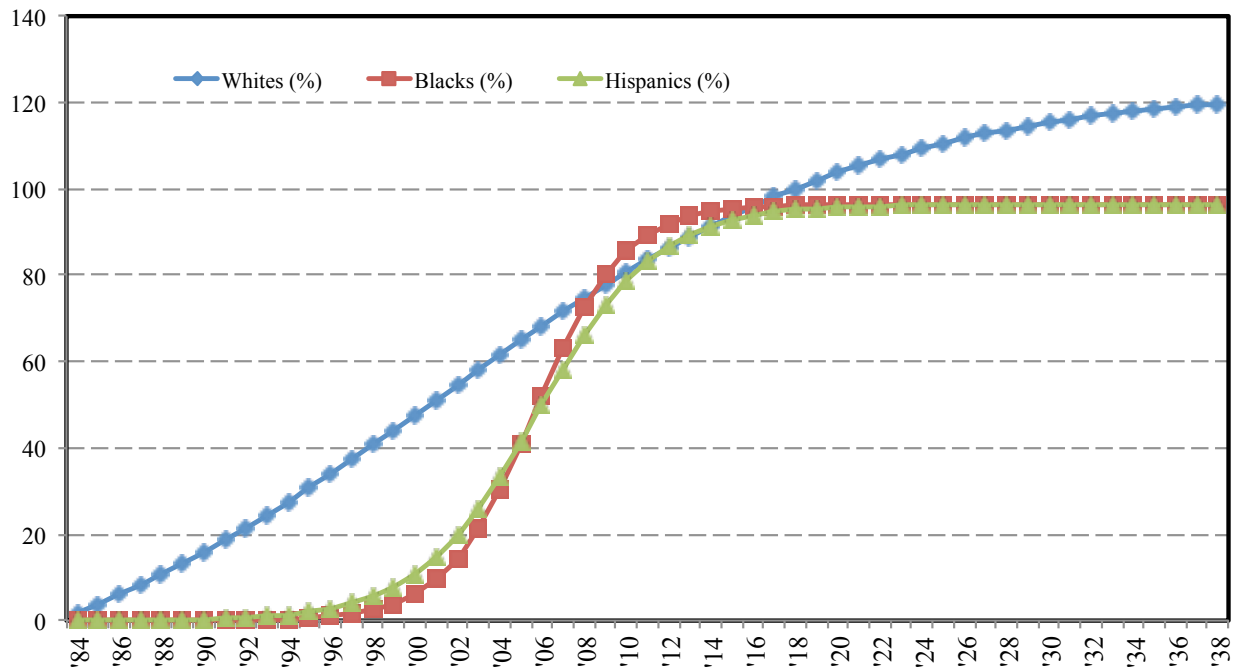
Figure # 2: Bass' Diffusion Growth for Cellphones Ownership (Pew Research Center)
